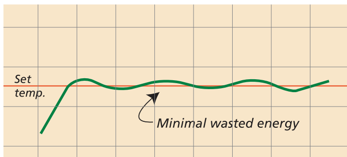
Digital Inverter
